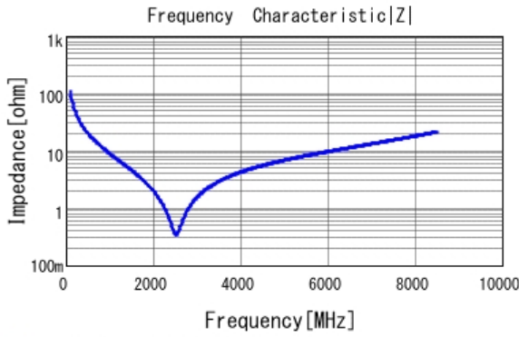
■ GRM0335C1H150JA01 |Z| DCOV, 25degC
