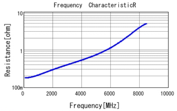
■ GRM0335C1H150JA01 R DCOV, 25degC
