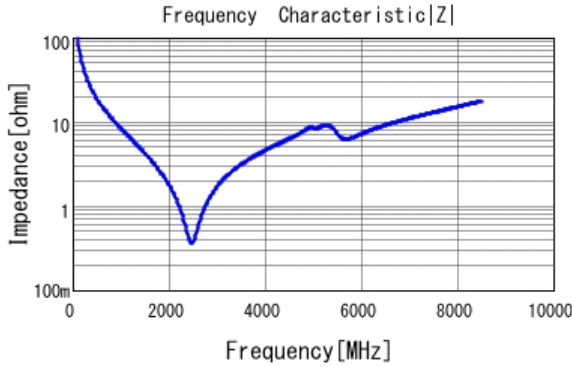
■ GRM0335C1H160GA01 |Z| DCOV, 25degC
