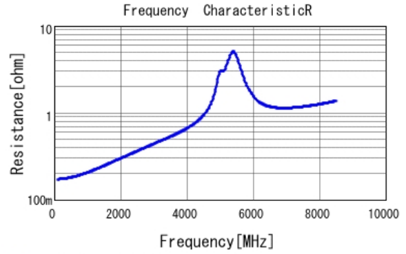
■ GRM0335C1H160JA01 R DCOV, 25degC
