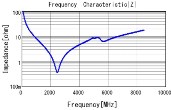
■ GRM0335C1H160JA01 |Z| DCOV, 25degC
