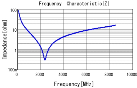
■ GRM0335C1H180JA01 |Z| DCOV, 25degC
