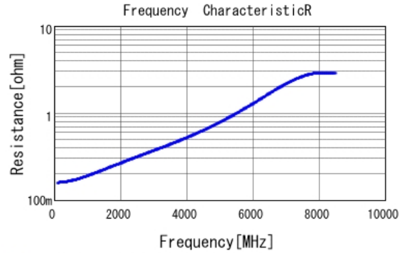
■ GRM0335C1H180JA01 R DCOV, 25degC
