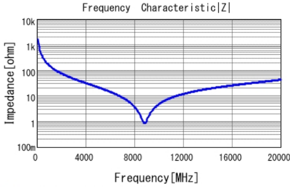
■ GRM0335C1H1R0CA01 |Z| DCOV, 25degC
