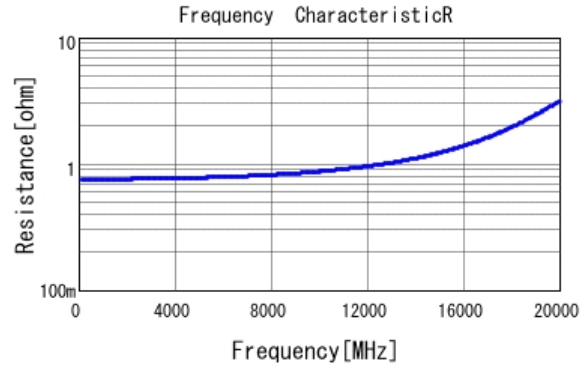
■ GRM0335C1H1R0CA01 R DCOV, 25degC
