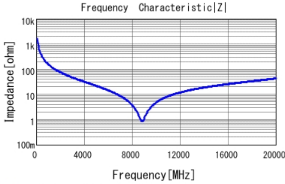
■ GRM0335C1H1R0WA01 |Z| DCOV, 25degC
