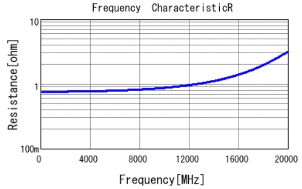
■ GRM0335C1H1R0WA01 R DCOV, 25degC
