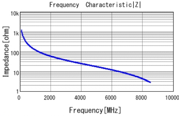
■ GRM0335C1H1R3BA01 |Z| DCOV, 25degC
