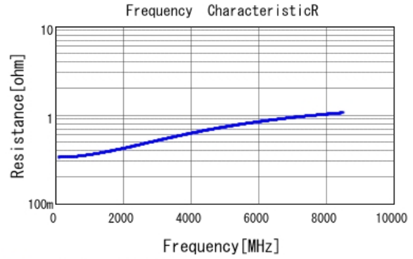
■ GRM0335C1H1R3BA01 R DCOV, 25degC
