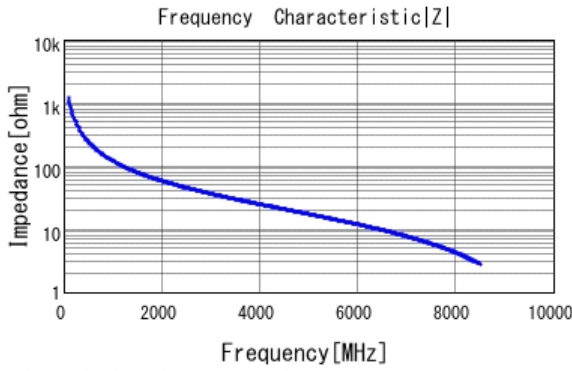
■ GRM0335C1H1R3CA01 |Z| DCOV, 25degC
