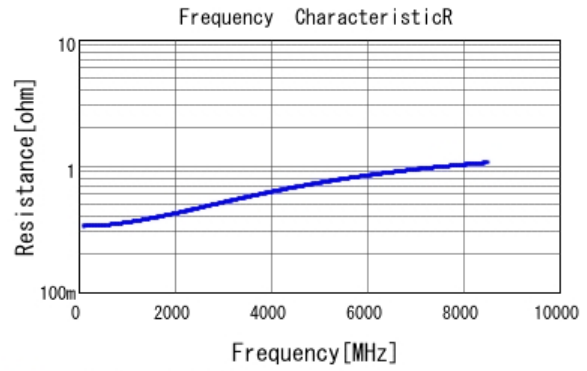
■ GRM0335C1H1R3CA01 R DCOV, 25degC
