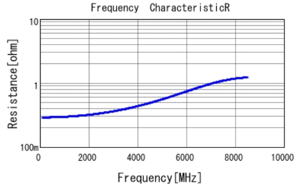
■ GRM0335C1H1R5CA01 R DC0V, 25degC
