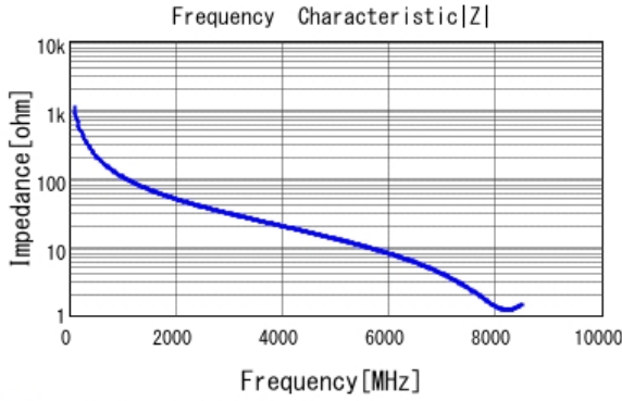
■ GRM0335C1H1R5CA01 |Z| DC0V, 25degC
