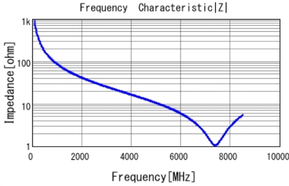
■ GRM0335C1H1R8BA01 |Z| DCOV, 25degC
