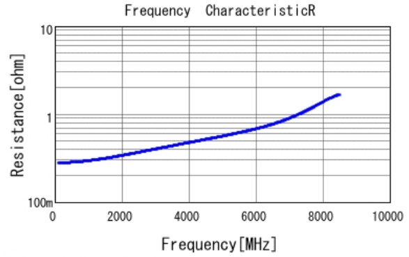
■ GRM0335C1H1R8BA01 R DCOV, 25degC
