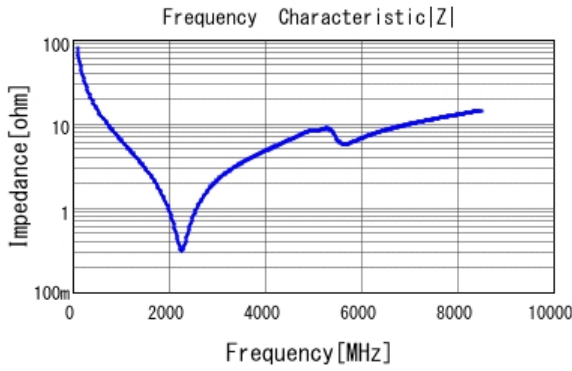
■ GRM0335C1H200GA01 |Z| DCOV, 25degC
