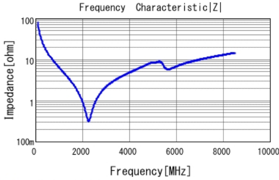
■ GRM0335C1H200JA01 |Z| DCOV, 25degC
