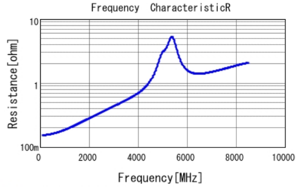
■ GRM0335C1H200JA01 R DCOV, 25degC
