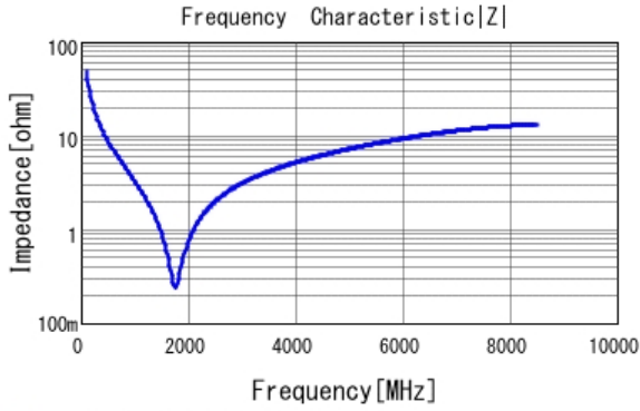
■ GRM0335C1H330GA01 |Z| DCOV, 25degC
