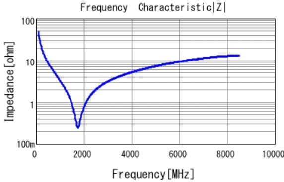
■ GRM0335C1H330JA01 |Z| DCOV, 25degC
