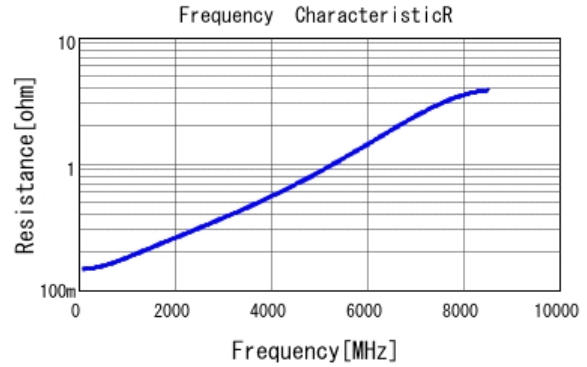
■ GRM0335C1H330JA01 R DCOV, 25degC
