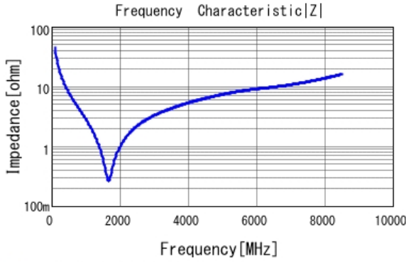
■ GRM0335C1H360GA01 |Z| DCOV, 25degC
