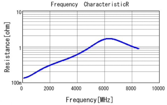
■ GRM0335C1H360GA01 R DCOV, 25degC
