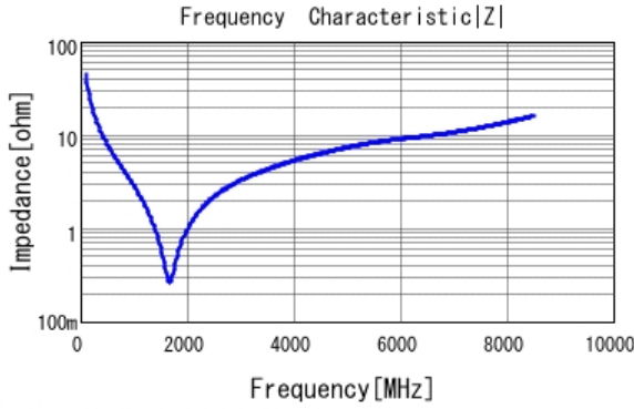
■ GRM0335C1H360JA01 |Z| DCOV, 25degC
