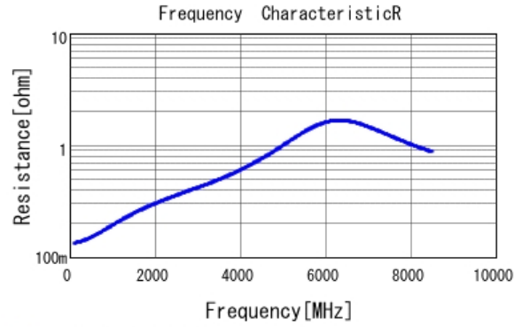
■ GRM0335C1H360JA01 R DCOV, 25degC
