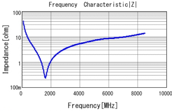
■ GRM0335C1H390GA01 |Z| DCOV, 25degC
