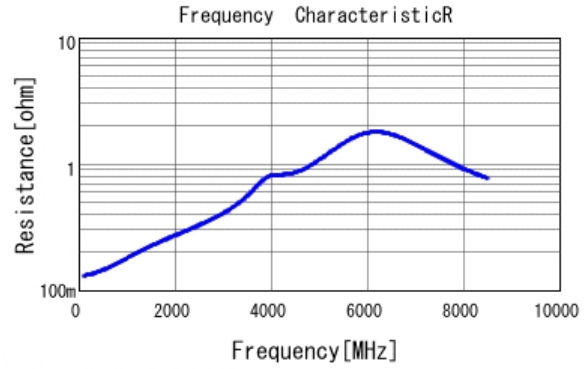
■ GRM0335C1H390GA01 R DCOV, 25degC
