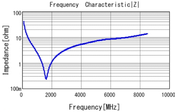
■ GRM0335C1H390JA01 |Z| DCOV, 25degC
