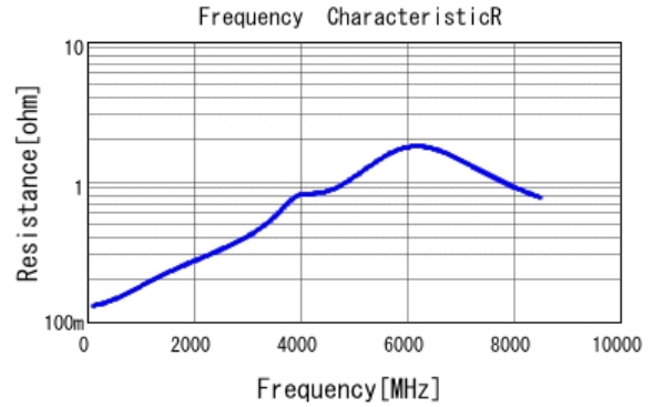
■ GRM0335C1H390JA01 R DCOV, 25degC
