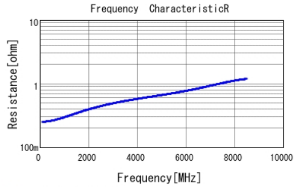
■ GRM0335C1H3R0BA01 R DCOV, 25degC
