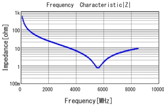
■ GRM0335C1H3R0BA01 |Z| DCOV, 25degC
