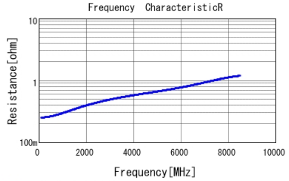
■ GRM0335C1H3R0CA01 R DCOV, 25degC
