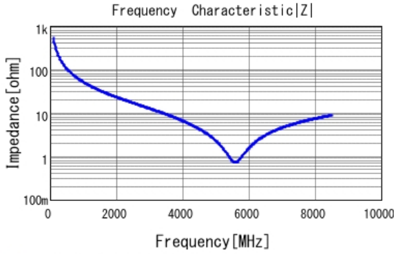
■ GRM0335C1H3R0CA01 |Z| DCOV, 25degC
