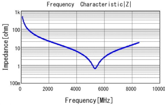
■ GRM0335C1H3R3CA01 |Z| DCOV, 25degC
