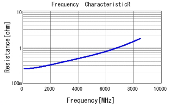
■ GRM0335C1H3R3CA01 R DCOV, 25degC
