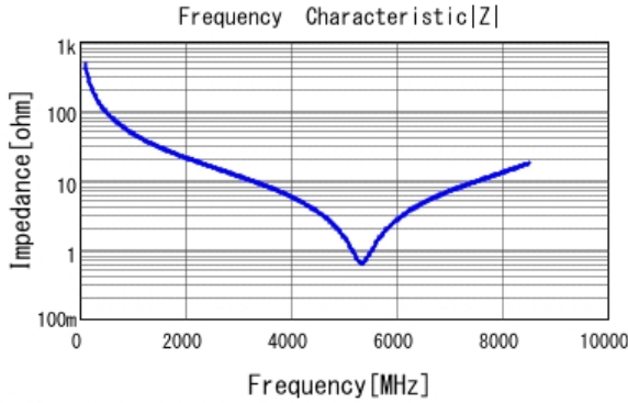
■ GRM0335C1H3R3WA01 |Z| DCOV, 25degC
