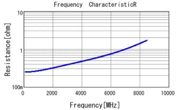
■ GRM0335C1H3R3WA01 R DCOV, 25degC
