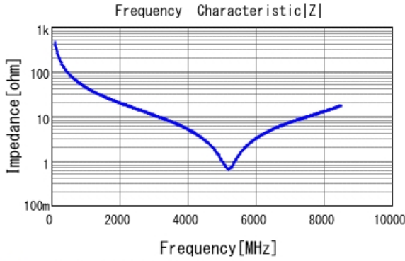
■ GRM0335C1H3R5BA01 |Z| DCOV, 25degC
