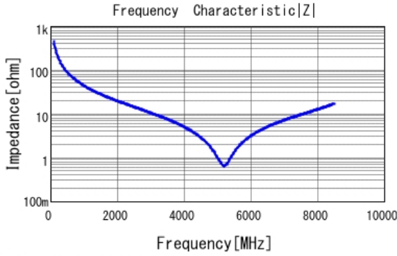
■ GRM0335C1H3R5WA01 |Z| DCOV, 25degC
