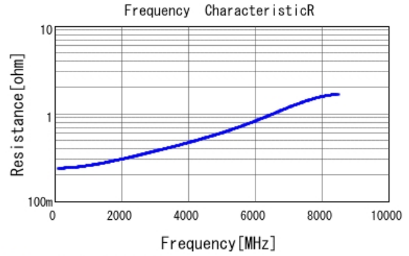
■ GRM0335C1H3R5WA01 R DCOV, 25degC
