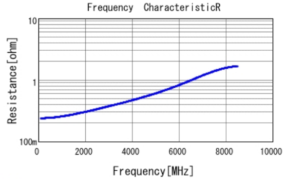
■ GRM0335C1H3R6BA01 R DCOV, 25degC
