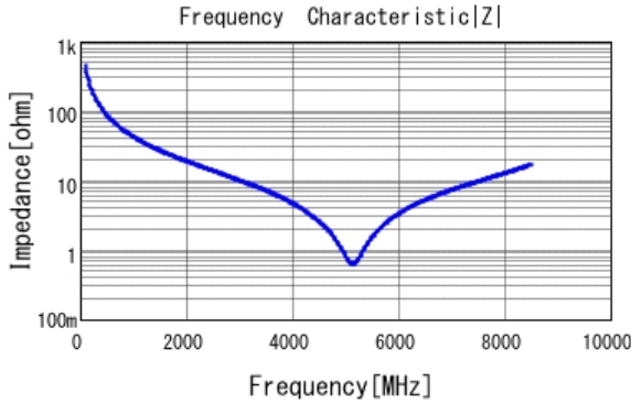
■ GRM0335C1H3R6BA01 |Z| DCOV, 25degC
