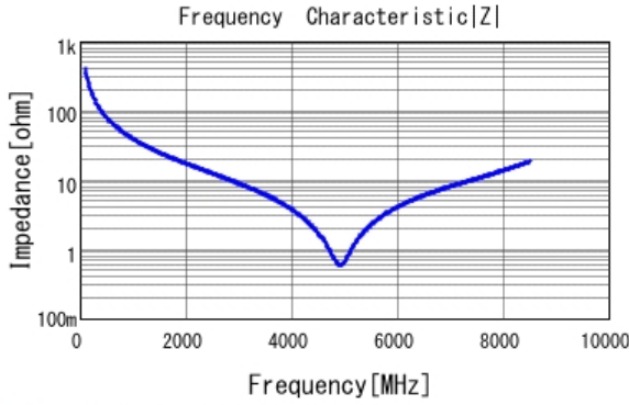
■ GRM0335C1H3R9CA01 |Z| DCOV, 25degC
