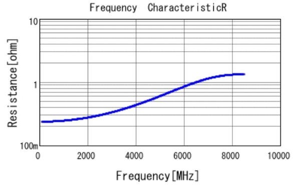
■ GRM0335C1H3R9CA01 R DCOV, 25degC
