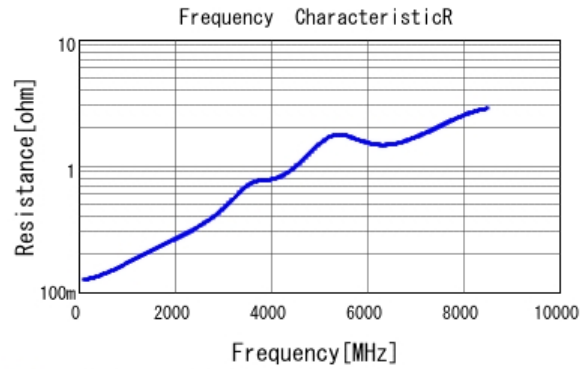
■ GRM0335C1H470JA01 R DCOV, 25degC
