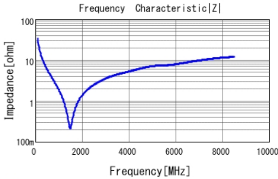
■ GRM0335C1H470JA01 |Z| DCOV, 25degC
