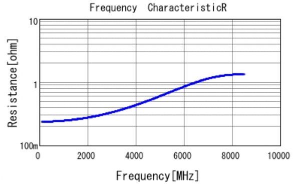
■ GRM0335C1H4R0BA01 R DCOV, 25degC
