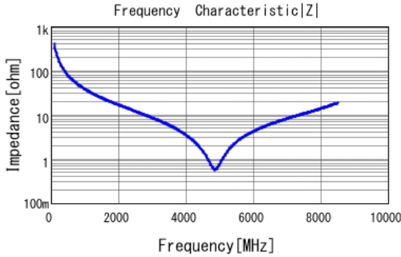
■ GRM0335C1H4R0BA01 |Z| DCOV, 25degC
