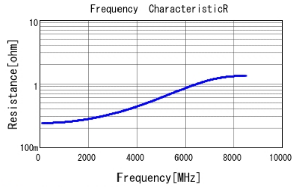
■ GRM0335C1H4R0CA01 R DCOV, 25degC
