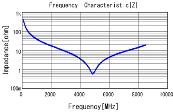
■ GRM0335C1H4R0CA01 |Z| DCOV, 25degC
