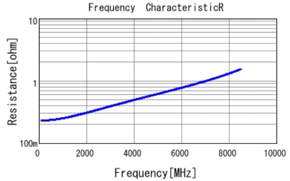
■ GRM0335C1H4R3BA01 R DCOV, 25degC
