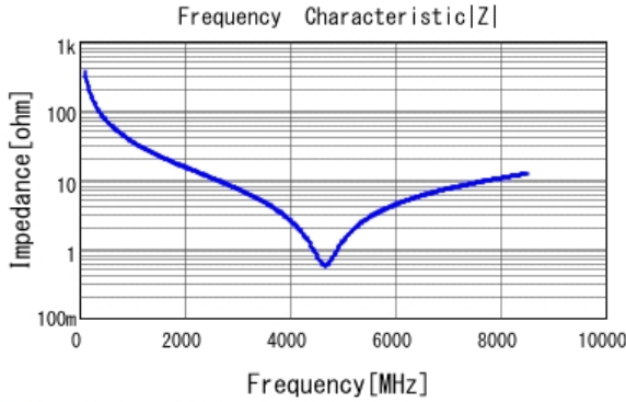
■ GRM0335C1H4R3BA01 |Z| DCOV, 25degC
