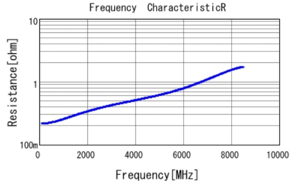
■ GRM0335C1H4R7CA01 R DCOV, 25degC
