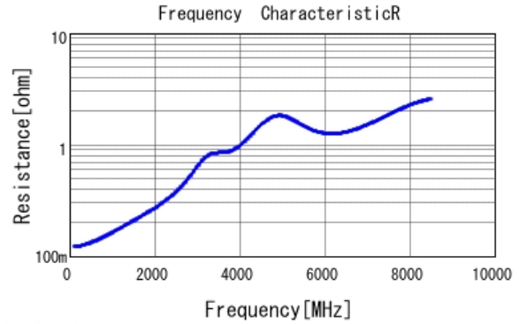
■ GRM0335C1H560GA01 R DCOV, 25degC
