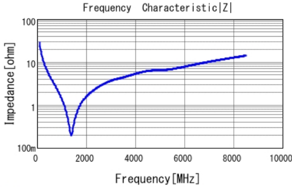
■ GRM0335C1H560GA01 |Z| DCOV, 25degC
