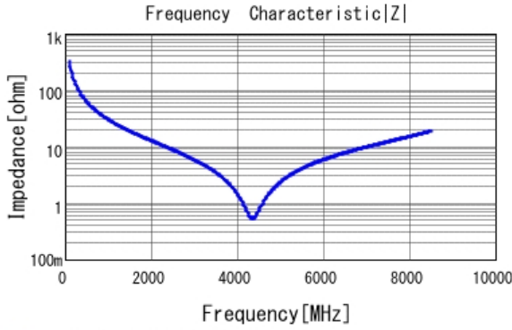
■ GRM0335C1H5R0BA01 |Z| DCOV, 25degC
