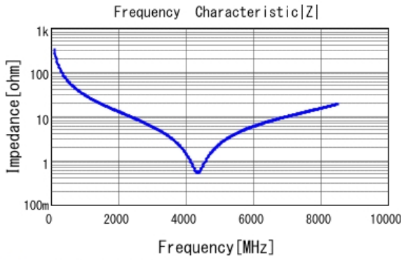
■ GRM0335C1H5R0CA01 |Z| DCOV, 25degC
