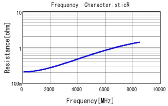
■ GRM0335C1H5R0CA01 R DCOV, 25degC
