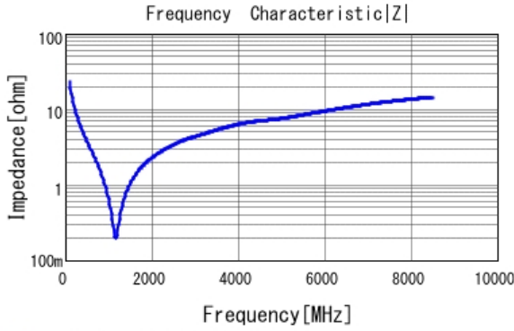
■ GRM0335C1H680GA01 |Z| DCOV, 25degC
