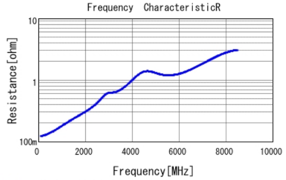
■ GRM0335C1H680GA01 R DCOV, 25degC
