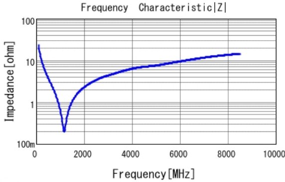
■ GRM0335C1H680JA01 |Z| DCOV, 25degC
