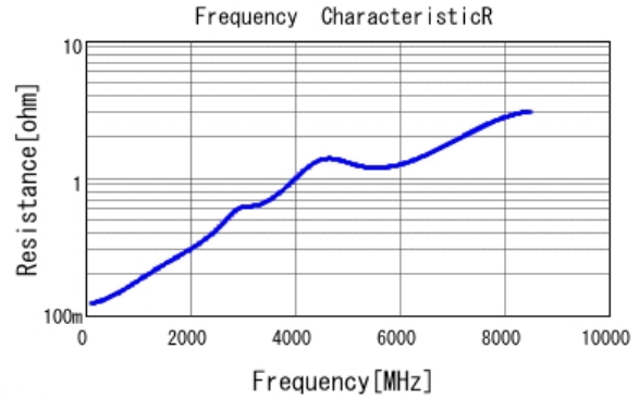
■ GRM0335C1H680JA01 R DCOV, 25degC
