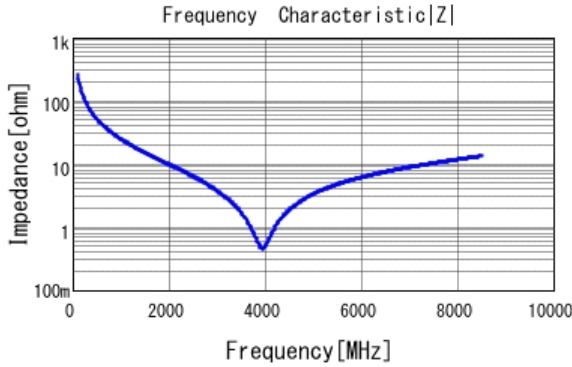
■ GRM0335C1H6R0BA01 |Z| DCOV, 25degC
