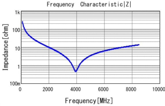
■ GRM0335C1H6R0DA01 |Z| DCOV, 25degC
