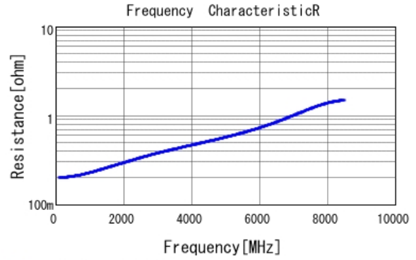
■ GRM0335C1H6R0DA01 R DCOV, 25degC
