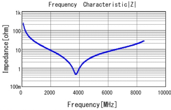
■ GRM0335C1H6R8CA01 |Z| DCOV, 25degC
