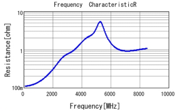
■ GRM0335C1H750GA01 R DCOV, 25degC
