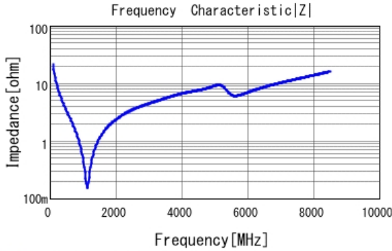
■ GRM0335C1H750GA01 |Z| DCOV, 25degC
