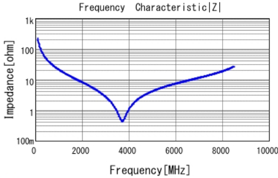
■ GRM0335C1H7R0CA01 |Z| DCOV, 25degC
