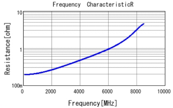
■ GRM0335C1H7R0CA01 R DCOV, 25degC
