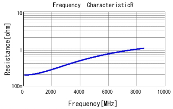
■ GRM0335C1H7R5CA01 R DC0V, 25degC
