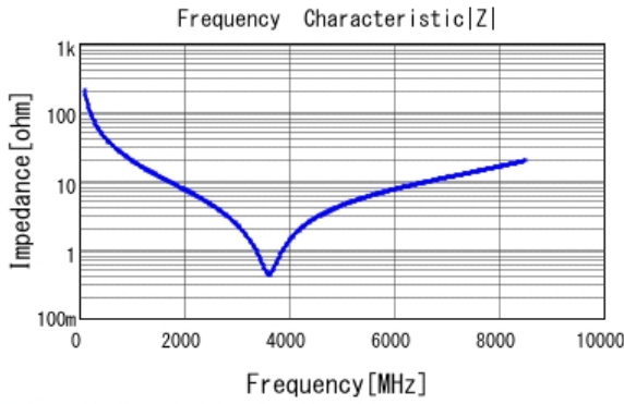
■ GRM0335C1H7R5CA01 |Z| DC0V, 25degC
