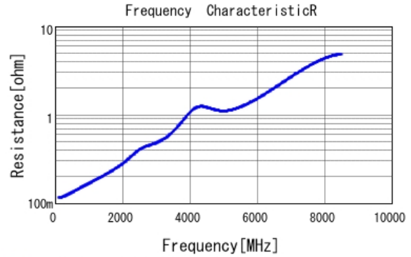
■ GRM0335C1H820GA01 R DCOV, 25degC
