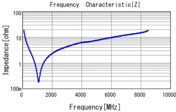
■ GRM0335C1H820GA01 |Z| DCOV, 25degC
