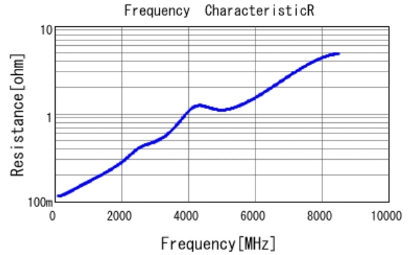
■ GRM0335C1H820JA01 R DCOV, 25degC
