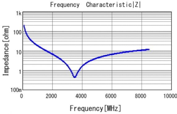
■ GRM0335C1H8R0BA01 |Z| DCOV, 25degC
