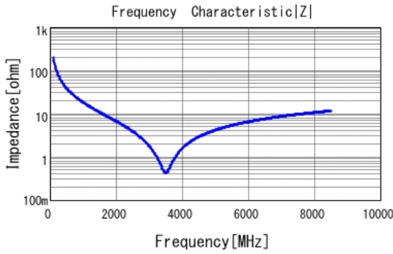
■ GRM0335C1H8R0CA01 |Z| DCOV, 25degC
