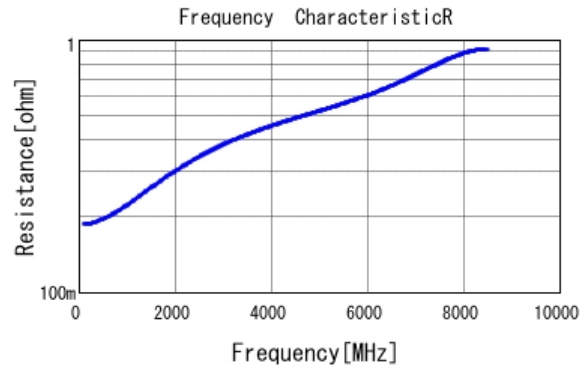
■ GRM0335C1H8R0CA01 R DCOV, 25degC
