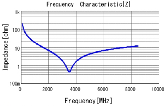
■ GRM0335C1H8R0DA01 |Z| DCOV, 25degC
