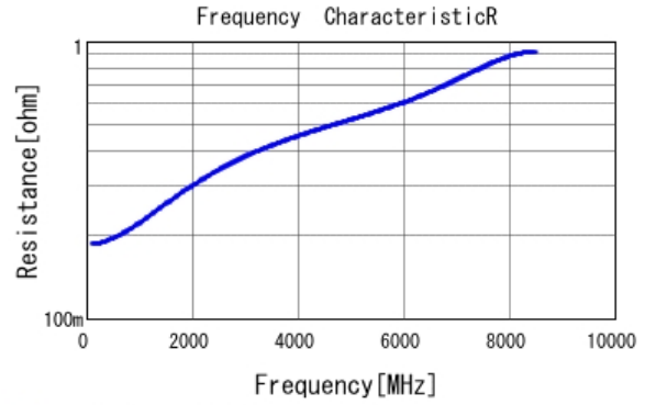
■ GRM0335C1H8R2BA01 R DCOV, 25degC
