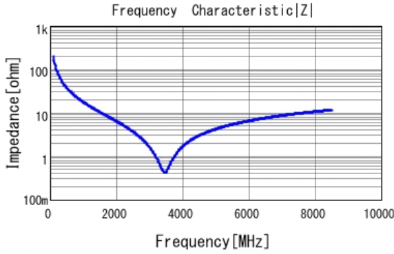
■ GRM0335C1H8R2BA01 |Z| DCOV, 25degC
