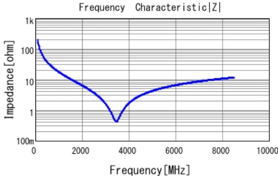
■ GRM0335C1H8R2DA01 |Z| DCOV, 25degC
