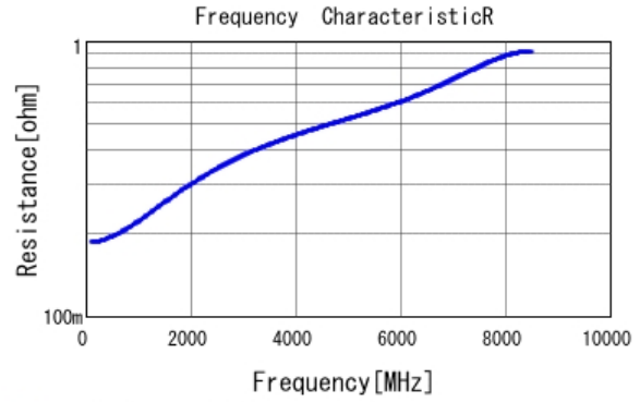
■ GRM0335C1H8R2DA01 R DCOV, 25degC
