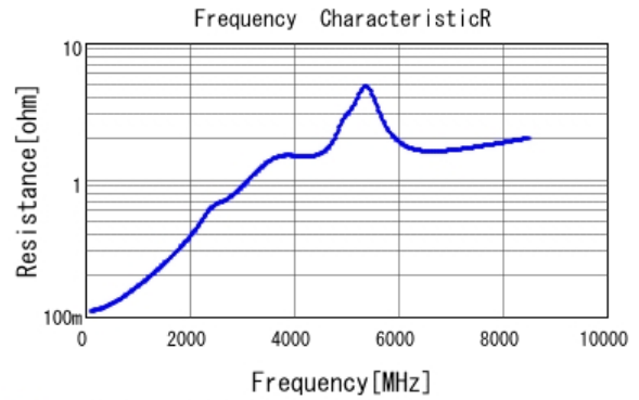
■ GRM0335C1H910GA01 R DCOV, 25degC
