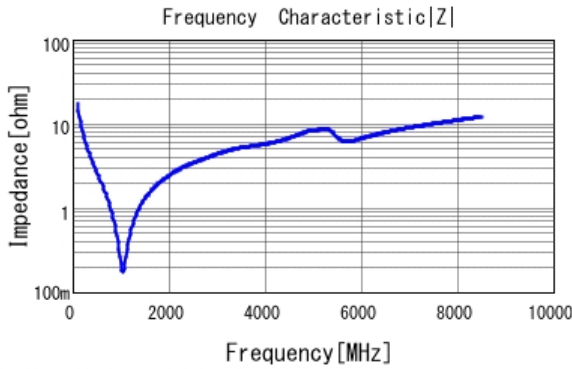
■ GRM0335C1H910GA01 |Z| DCOV, 25degC
